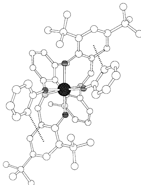
Fig. 6 Molecular structure of [\text{ZrL}^1(\text{OPh})_2] 9 (non-hydrogen atoms) viewed along the approximate \text{C}_2 axis and indicating the arene edge-face interactions.
