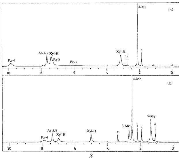
Fig. 3 400 MHz ^1\text{H} NMR spectra of (a) [\text{Cu}_2(\text{L})_2(\text{OClO}_3)_2] 1 and (b) [\text{Cu}_2(\text{L}')_2(\text{OClO}_3)_2] 2 at room temperature in \text{CD}_3\text{CN} solution. The peaks marked e, i and s are due to diethyl ether, impurity and solvent, respectively. The abbreviations (Ar, Pz and Xyl) used in the assignments denote aromatic ring, pyrazole ring and xylyl protons respectively.
