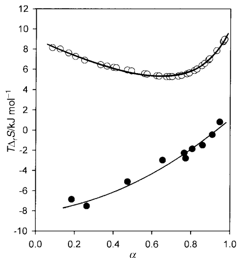
Fig. 9 Variation of T\Delta_r S with \alpha , the fraction of exchanged \text{Cl}^- , for the two processes studied here: \text{Cl}^- - \text{OH}^- exchange ( \circ ); \text{Cl}^- - \text{NO}_3^- exchange ( \bullet ).
