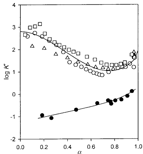
Fig. 6 Variation of K' , the apparent partition constant, with \alpha , the fraction of exchanged \text{Cl}^- , for the two processes studied here: \text{Cl}^- – \text{OH}^- exchange on 30.3 ( \Delta ), 50.1 ( \circ ) and 73.9 mg ( \square ) of LDH; \text{Cl}^- – \text{NO}_3^- exchange on 15.6 mg of LDH ( \bullet ).
