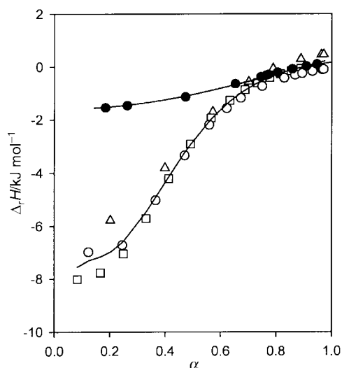
Fig. 8 Variation of the derivative, dQ/dn_{\text{Cl}^{-}_{\text{aq}}} , i.e. the molar enthalpy of reaction \Delta_r H , with \alpha , the fraction of exchanged \text{Cl}^- , for the two processes studied here: \text{Cl}^- - \text{OH}^- exchange on 3.0 ( \Delta ), 5.2 ( \circ ) and 7.3 mg ( \square ) of LDH; \text{Cl}^- - \text{NO}_3^- exchange on 5.2 mg of LDH ( \bullet ).
