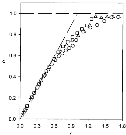
Fig. 5 \text{Cl}^- – \text{OH}^- exchange isotherms: variation of \alpha , the fraction of exchanged \text{Cl}^- , with r , the ratio of the total number of moles of \text{OH}^- over the total number of moles of \text{Cl}^- present in the two phases at equilibrium, for various amounts of LDH [( \Delta ) 30.3; ( \circ ) 50.1 and ( \square ) 73.9 mg].
