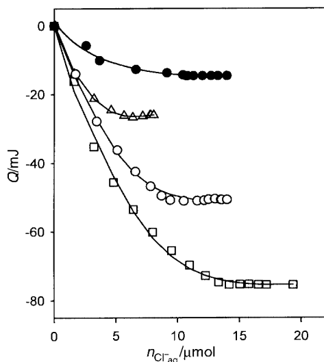
Fig. 7 Variation of the cumulative heat value at each calorimetric titration step with the corresponding number of moles of exchanged chloride deduced from the \text{Cl}^- - \text{OH}^- exchange isotherms, for three experiments involving different amounts of LDH [ (\Delta) 3.0; (\circ) 5.2 and (\square) 7.3 mg], and from the \text{Cl}^- - \text{NO}_3^- exchange isotherm [ (\bullet) 5.2 mg of LDH].
