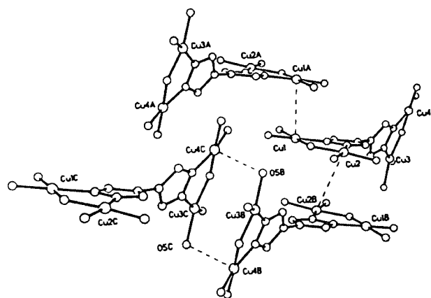
Fig. 2 (a) Molecular structure and atomic numbering scheme for 2 . Thermal ellipsoids are shown at the 40% level. (b) The coordination chromophores and bridging ligand (mdpz, methyl groups omitted for clarity) of 2 showing the intermolecular stacking association of Cu(1) and Cu(2) with Cu(1A) and Cu(2B), respectively and of Cu(3B) and Cu(4B) with Cu(4C) and Cu(3C), respectively.
