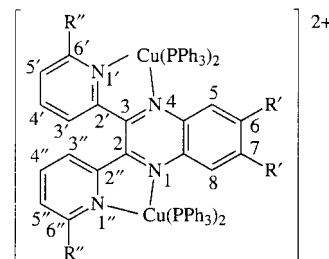
Fig. 1 Ligands and numbering scheme: R'' = R' = H, 1; R'' = H, R' = benzo, 2; R'' = H, R' = CH 3 , 3; R'' = H, R' = Cl, 4; R'' = CH 3 , R' = H, 5; R'' = CH 3 , R' = benzo, 6; R'' = CH 3 , R' = CH 3 , 7; R'' = CH 3 , R' = Cl, 8.
