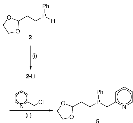
Scheme 3 Synthesis of phosphine 5 . (i) n -BuLi, THF, -80 to 0 °C, 30 min, -n -BuH; (ii) hexanes, -30 to 20 °C, 1.5 h, -\text{LiCl} .
