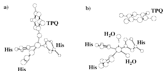
Fig. 1 Views of the TPQ-on (a) and TPQ-off (b) forms of the active site of copper amine oxidase. For simplicity, only the methylene carbon atom of the cofactor is shown.
