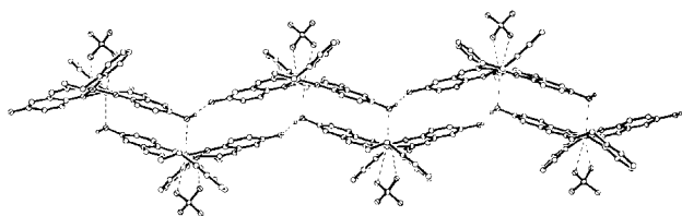
Fig. 3 Partial packing diagram of the structure of [\{Cu(\mu-L)\}]_2\cdot[BF_4]_2\cdot MeNO_2 ( 1\cdot MeNO_2 ), showing the 'dimer of chains' packing motif. For clarity, all C-bound H atoms, and the non-co-ordinated anion and solvent molecule, have been omitted.
