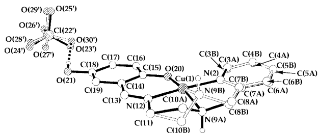
Fig. 5 View of the asymmetric unit in the structure of [CuL 2 ]ClO 4 2 , showing the atom numbering scheme employed. Both the major (solid bonds) and minor (hollow bonds) disorder orientations for the cation and anion are shown. Primed atoms are related to unprimed atoms by the relation by 1 - x , -\frac{1}{2} + y , \frac{1}{2} - z . For clarity, all C-bound H atoms have been omitted.
