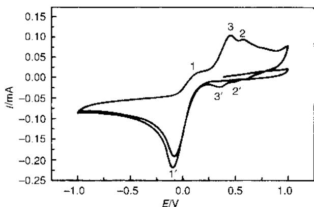
Fig. 3 Cyclic voltammograms of [RuCl 3 (dppb)(4-pic)], 1.0 \times 10^{-3} mol l -1 , in CH 2 Cl 2 with 0.1 mol l -1 NBu 4 ClO 4 , scan rate 100 mV s -1 , measured at a platinum electrode.
