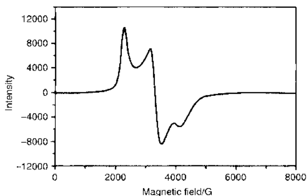
Fig. 1 EPR spectrum of [\text{RuCl}_3(\text{dppb})(4\text{-pic})] (X band frequency) at -160 \text{ }^\circ\text{C} in the solid state.
