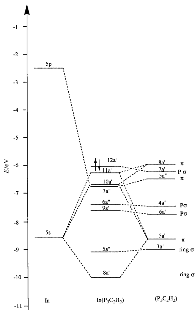
Fig. 4 MO diagram for I , [\text{In}(\eta^5\text{-P}_3\text{C}_2\text{H}_2)] .
