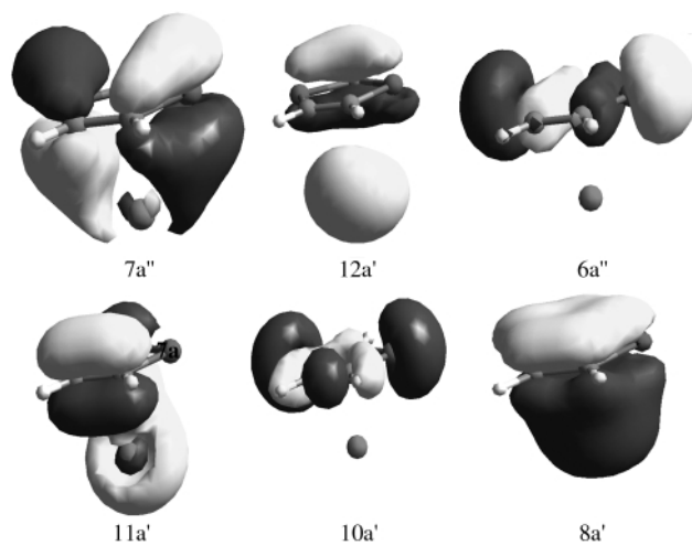
Fig. 7 Highest occupied orbitals of II, [\text{In}(\eta^5\text{-P}_2\text{C}_3\text{H}_3)] .
