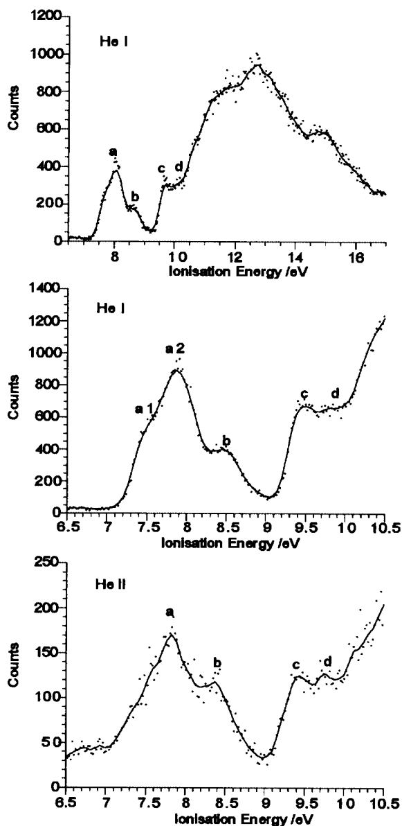
Fig. 3 He I and He II PE spectra of 2 , [\text{In}(\eta^5\text{-P}_2\text{C}_3\text{Bu}_3)] .
