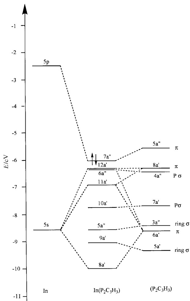
Fig. 5 MO diagram for II, [\text{In}(\eta^5\text{-P}_2\text{C}_3\text{H}_3)] .
