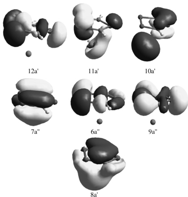
Fig. 6 Highest occupied orbitals of I, [\text{In}(\eta^5\text{-P}_3\text{C}_2\text{H}_2)] .
