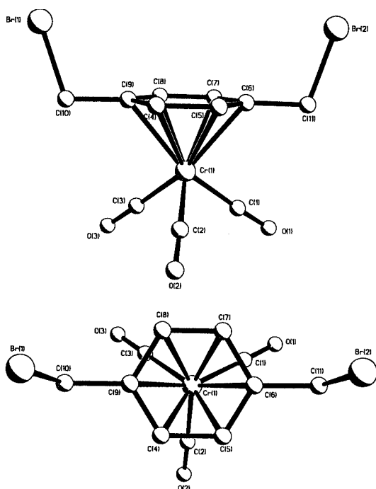
Fig. 5 Molecular structure of complex 8 .
