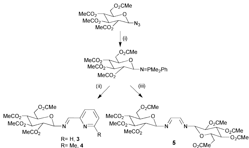
Scheme 1 (i) +PMe 2 Ph, -N 2 ; (ii) +6-R-C 5 H 3 NCHO-2, -O=PMe 2 Ph; (iii) +0.5 OHCCCHO, -O=PMe 2 Ph.
