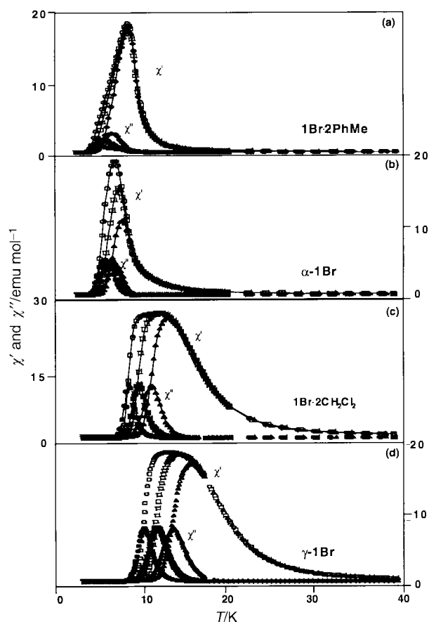
Fig. 5 Temperature dependencies of the dispersive, \chi' ( \times , \blacksquare , and \ominus ) and absorptive, \chi'' ( \times , \blacksquare , and \circ ), components of the ac susceptibility at 10, 10 2 , and 10 3 Hz, respectively, (a) 1Br·2PhMe , (b) \alpha - 1Br , (c) 1Br·2CH 2 Cl 2 , and (d) \gamma - 1Br . ( H_{\text{dc}} = 0 Oe, amplitude = 1 Oe.) Samples were zero-field cooled and data taken upon warming.
