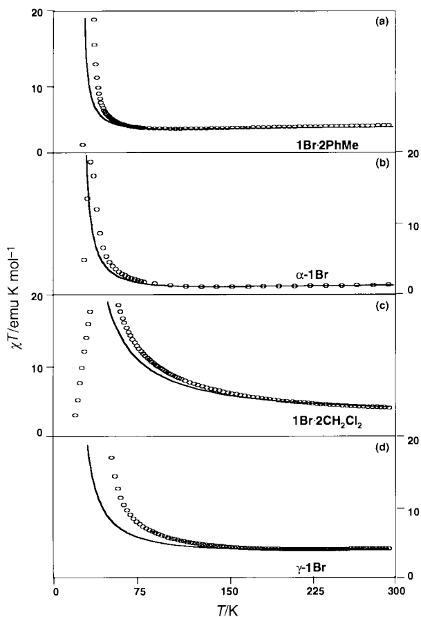
Fig. 4 Fit of the \chi T(T) data to the Seiden expression 19 for (a) 1Br·2PhMe , (b) \alpha - 1Br , (c) 1Br·2CH 2 Cl 2 , and (d) \gamma - 1Br .
