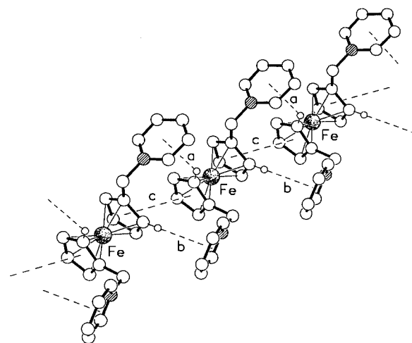
Fig. 5 One of the C–H... \pi and \pi – \pi linked chains of molecules present in the structure of complex 2. The H... \pi distances ( \text{\AA} ) and C–H... \pi angles ( ^\circ ) are (a) 2.88, 138 and (b) 2.82, 152 . The centroid–centroid and mean interplanar separations (c) are 3.87 and 3.57 \text{ \AA} respectively.
