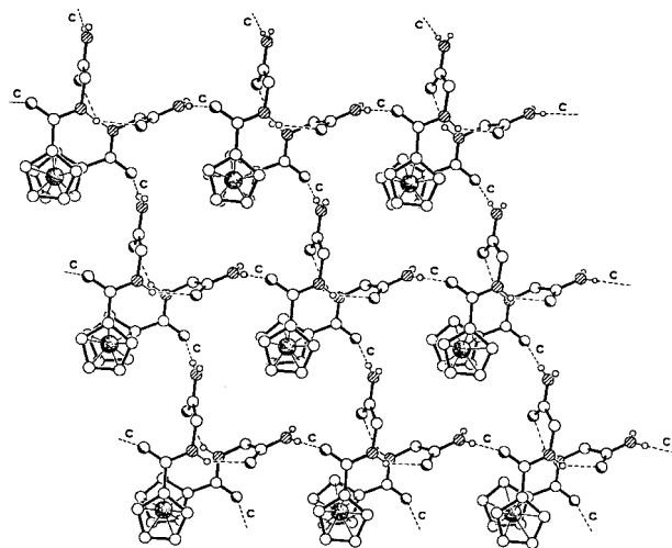
Fig. 2 One of the N-H \cdots O hydrogen bonded sheets of molecules present in the structure of complex 1 . The hydrogen bonding geometry is N \cdots O 2.94, H \cdots O 2.04 Å and N-H \cdots O 177^\circ .
