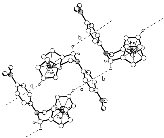
Fig. 7 One of the the C-H... \pi and \pi - \pi linked chains of molecules present in the structure of complex 4. The H... \pi distances (Å) and C-H... \pi angles (°) are (a) 2.92, 151 and (b) 3.05, 123.
