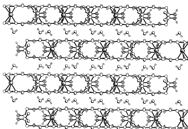
Fig. 3 The intercalation between the hydrogen bonded sheets in the structure of complex 1 by the solvent water molecules. The sheets are cross-linked by O-H \cdots O hydrogen bonds from these included water molecules (see text).
