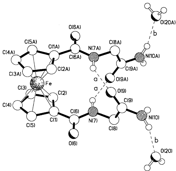
Fig. 1 The molecular structure of complex 1 . The hydrogen bonding geometries are N \cdots O , H \cdots O (Å), N-H \cdots O ( ^\circ ): (a) 2.88, 2.08, 147 and (b) 2.95, 2.08, 165.
