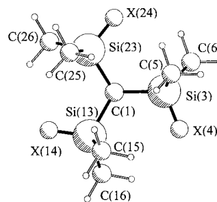
Fig. 2 Atom numbering scheme adopted for \text{CH}(\text{SiMe}_2\text{X})_3 ( \text{X} = \text{H} 1 or \text{Br} 2 ). The hydrogen atom \text{H}(2) attached to the central carbon is not shown.
