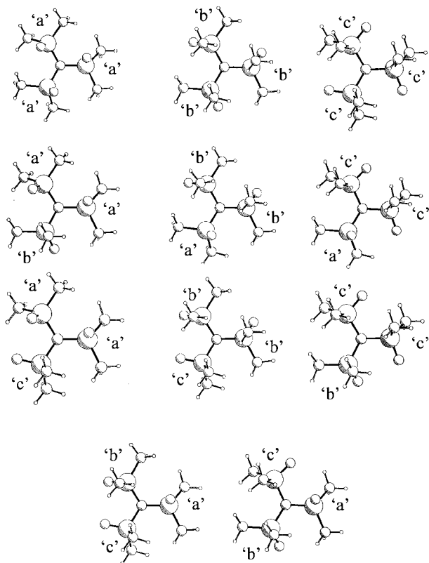
Fig. 1 Molecular structures of the eleven conformers of \text{CH}(\text{SiMe}_2\text{X})_3 ( \text{X} = \text{H} 1 or \text{Br} 2 ). The hydrogen atom attached to the central carbon [denoted \text{H}(2) in the text] is not shown. Torsional angles \text{H}(2)\text{-C}(1)\text{-Si-H} are denoted 'a' ca. 160^\circ , 'b' ca. 40^\circ and 'c' ca. -80^\circ .
