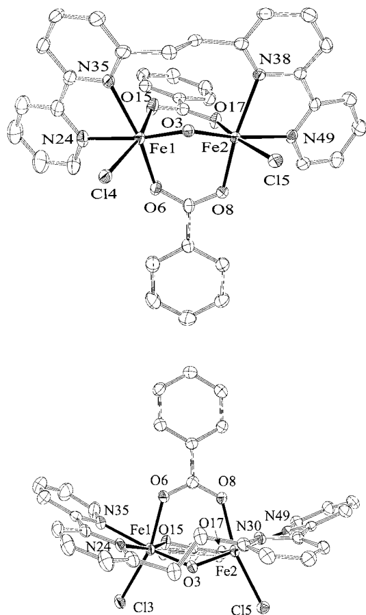
Fig. 2 ORTEP representation at the 50% probability level of [\text{Fe}_2\text{OCl}_2(\text{O}_2\text{CPh})_2\text{L}] 2 from two approximately perpendicular viewpoints to emphasize the bowing of the L ligand.
