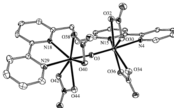
Fig. 6 ORTEP representation at the 50% probability level of [\text{Fe}_2\text{O}(\text{NO}_3)_4]^{4+} 7.
