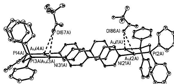
Fig. 1 A view of the structure of complex 8. Two distant trifluoroacetate ions are not shown.
