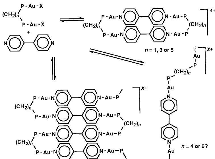
Scheme 3 P = \text{PPh}_2 .
