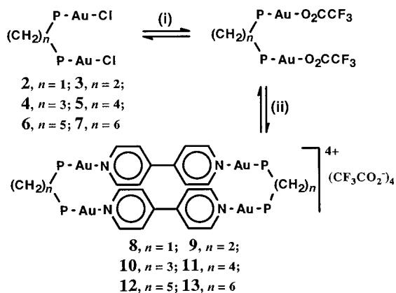
Scheme 2 P = \text{PPh}_2 . Reagents: (i) \text{AgO}_2\text{CCF}_3 , -\text{AgCl} ; (ii) 4,4'-bipyridine.
