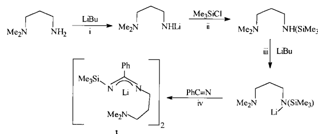
Scheme 1 Synthesis of the lithium amidinate [\text{Li}\{N(\text{SiMe}_3)\text{C}(\text{Ph})\text{N}(\text{CH}_2)_3\text{NMe}_2\}]_2 [ \equiv (\text{LiL})_2 ] 1 .
