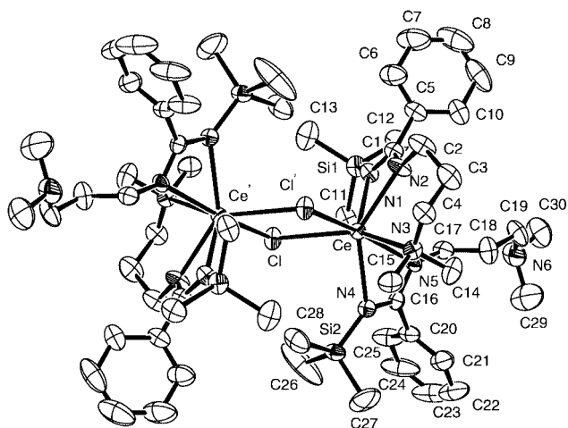
Fig. 3 The molecular structure of [\{\text{Ce}(\text{L})_2(\mu\text{-Cl})\}_2] \mathbf{5} .
