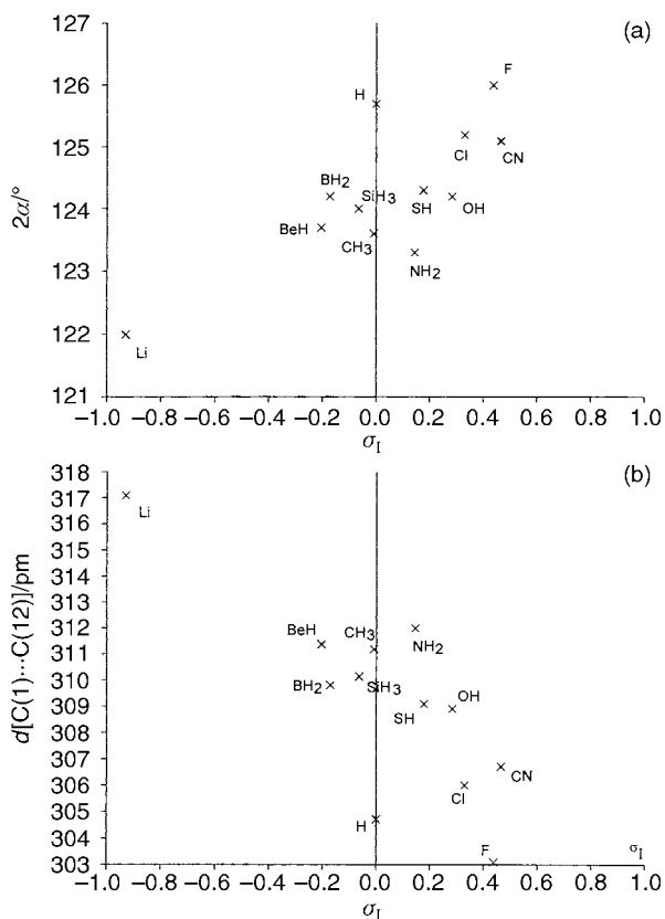
Fig. 5 (a) Plot of the angles 2\alpha (symmetrised where there is strictly no C_5 axis, see e.g. Table 6) against the theoretically calculated (MP2/6-31G*) inductive parameters \sigma_1 for 1,12-disubstituted 1,12-dicarbado-decaboranes. Also depicted is the reference point of the parent 1,12- C_2B_{10}H_{12} . The correlation coefficient r = 0.857 (excluding H, see text). (b) Plot of the body diagonals d[\text{C}(1)\cdots\text{C}(12)] against the theoretically calculated (MP2/6-31G*) inductive parameters \sigma_1 for 1,12-disubstituted 1,12-dicarbaboranes. The correlation coefficient r = -0.883 (excluding H, see text).
