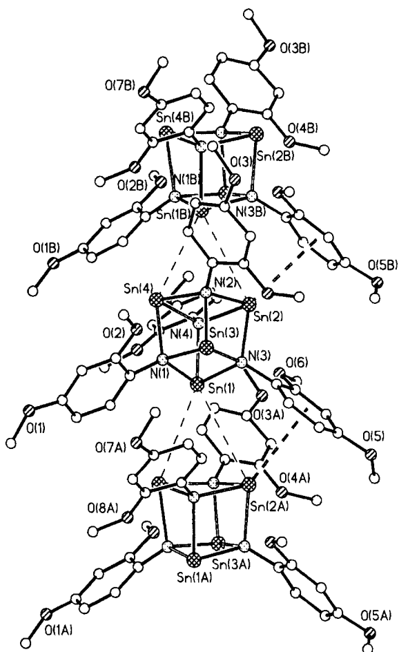
Fig. 6 Association of compound 6 in the crystal lattice into long chain polymers via Sn...Sn and Sn...O interactions between neighbouring molecules related by c -glide symmetry.
