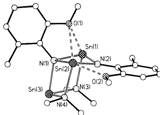
Fig. 7 The nido -cubane structure of [{SnN(2-MeO-6-MeC 6 H 3 ) 2 Sn(NMe 2 ) 2 ] 7 .
