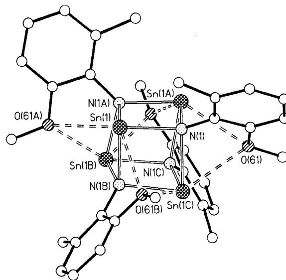
Fig. 3 The cubane structure of [SnN{2-MeO-6-MeOC 6 H 3 }] 4 3 .
