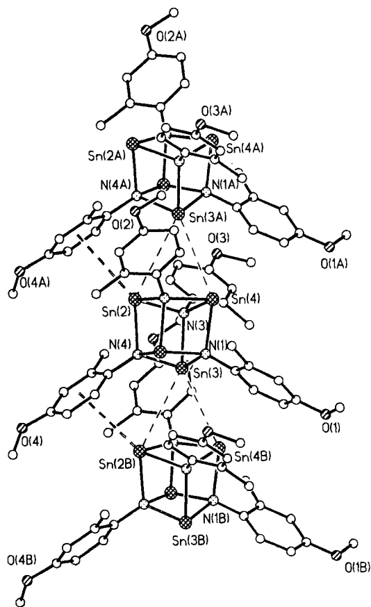
Fig. 2 Association of compound 2 in the crystal lattice into polymers via Sn...Sn and Sn... \eta^6 -aryl interactions between neighboring molecules related by c -glide symmetry.
