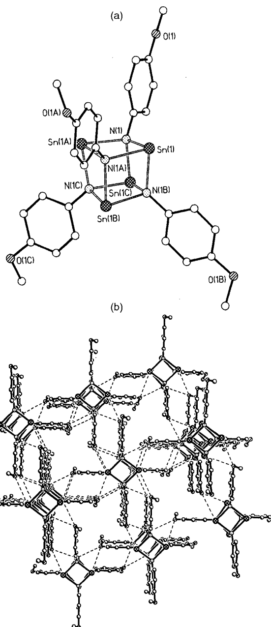
Fig. 1 (a) The cubane structure of [SnN{4-MeOC 6 H 4 }] 4 1 , which has crystallographic S 4 symmetry. (b) Association of 1 in the crystal lattice through 'face' Sn...O...Sn interactions.
