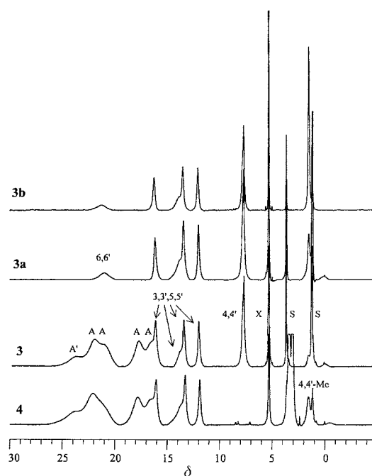
Fig. 3 ^1\text{H-NMR} spectra of complex 4 (bottom), 3 (second from bottom), 3a (third from bottom), and 3b (top). See text for experimental details and assignment of resonances. X = \text{CH}_2\text{Cl}_2 , S = \text{EtOH} solvent of crystallization.
