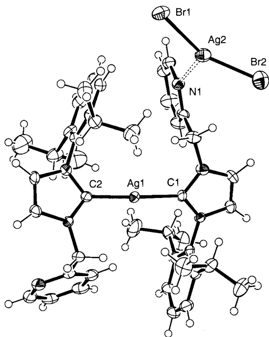
Fig. 1 An ORTEP 9 diagram of the crystal structure of silver carbene complex 7c (50% probability thermal ellipsoids, as in all cases shown).
