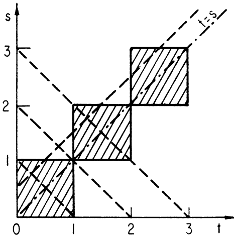
FIG. 2.—The (t, s) diagram for a random step-function. \Gamma\left(\xi - \frac{h}{2}, \xi + \frac{h}{2}\right) is periodic in \xi and for a translation parallel to t = s , \Gamma(t + 1, s + 1) = \Gamma(t, s) .
