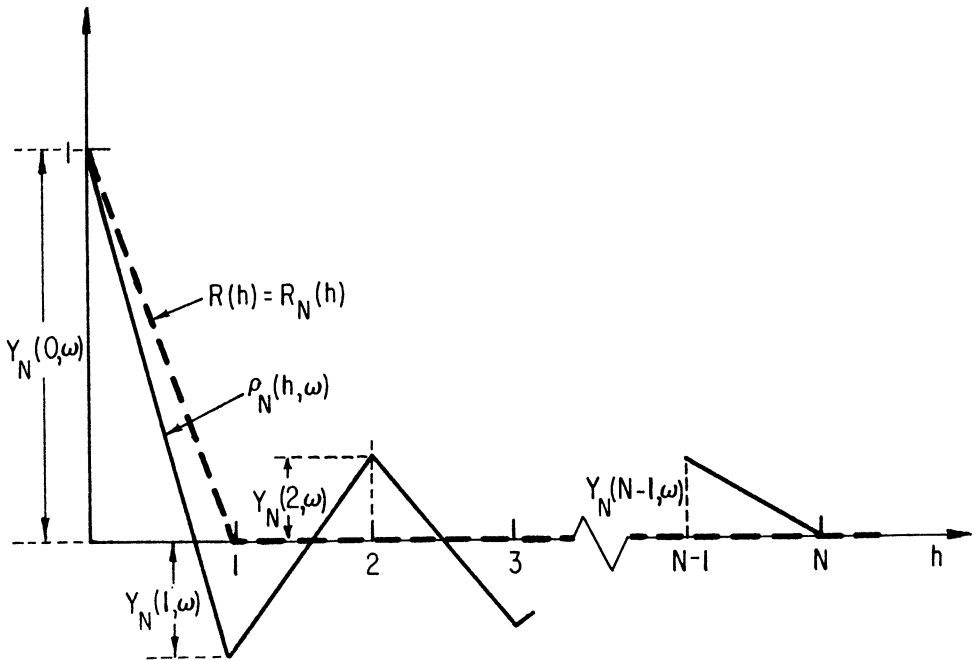
FIG. 3.—The polygonal line \rho_N(h, \omega) represents a sample-correlation of the step-function. R_N(h) = \overline{\rho_N(h, \omega)} is the sub-correlation, which for the step-function, is equal to the correlation function R(h) .
