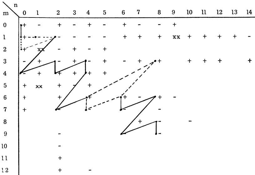
FIG. 4. The initial segment of the path of maximal convergence along with the sign of R_{n,m}(x) - \Gamma(x) at the leftmost extremal point of the error curve.
