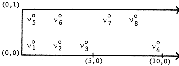
General location of common zeros, \lambda > 0
