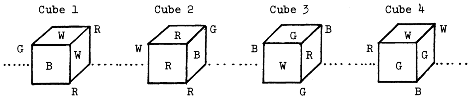
FIGURE 1. Instant Insanity cubes
