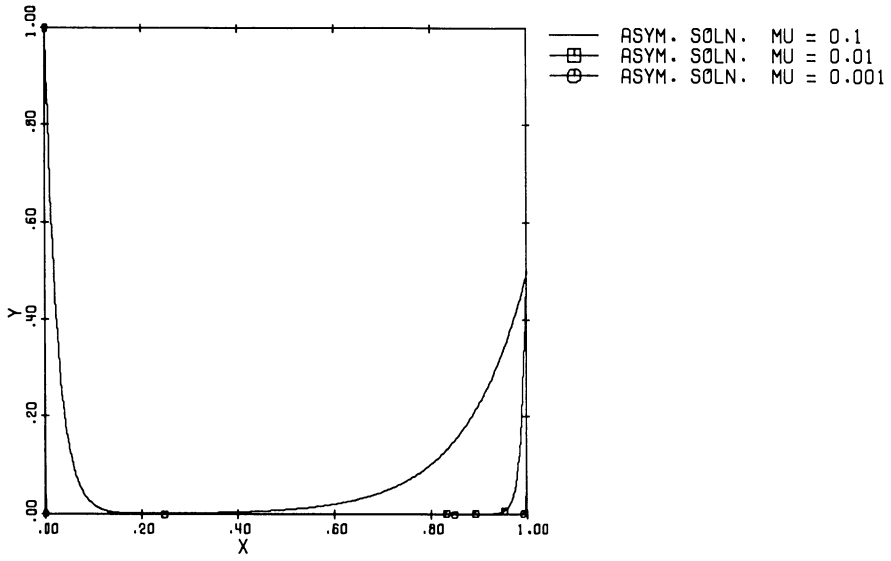
FIGURE 1 Asymptotic solution of Example 1a: \epsilon y'' + \mu y' - y = 0, y(0) = 1, y(1) = \frac{1}{2}, \epsilon = \mu^{5/2}
