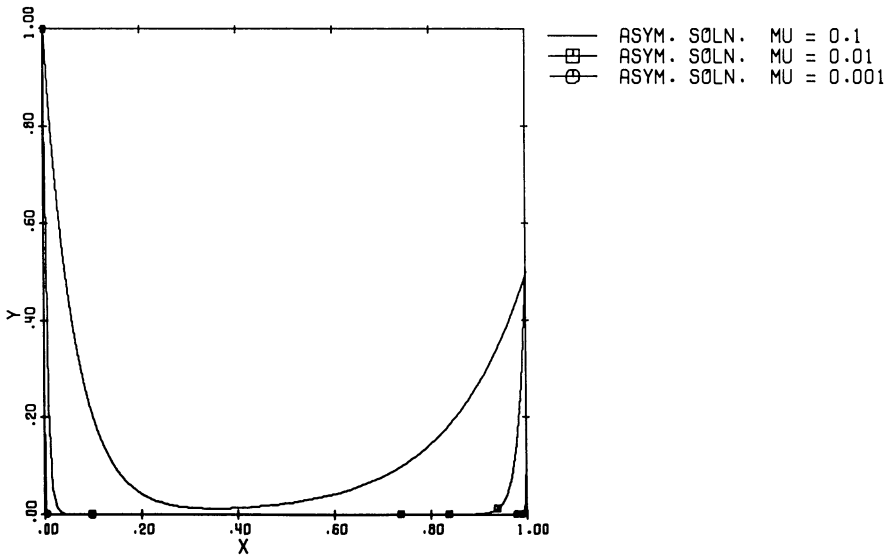
FIGURE 2 Asymptotic solution of Example 1b: \epsilon y'' + \mu y' - y = 0, y(0) = 1, y(1) = \frac{1}{2}, \epsilon = \mu^2
