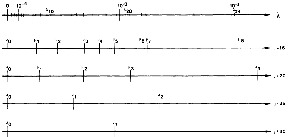
FIGURE 6.2 Eigenvalues \lambda_k and shifts \mu_s of test problem
