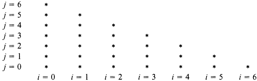
FIGURE 6-1: Random walk on a triangular grid
