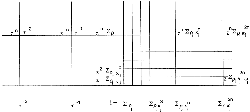
FIGURE 2.2 Normal modes of the solution
