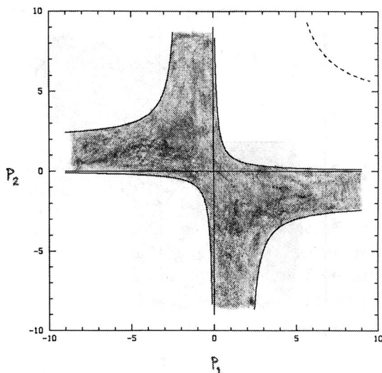
FIGURE 7 Stability regions for the ILU factorization.
