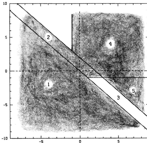
FIGURE 9 Values of x and y where inequality (6.1) holds.
