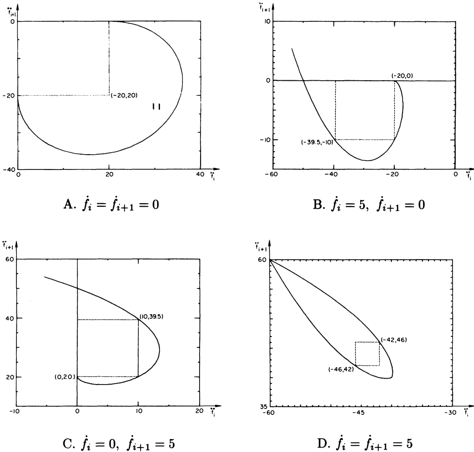
FIGURE 4.4 Four cross sections of the quintic monotonicity region.
