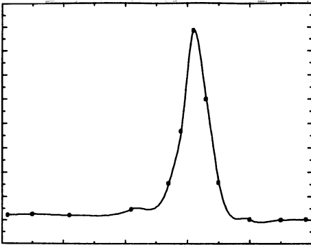
A. Unconstrained cubic
