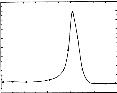
C. MC cubic
