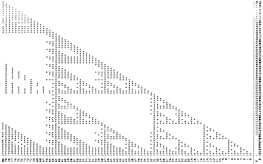
20-ary divisors
