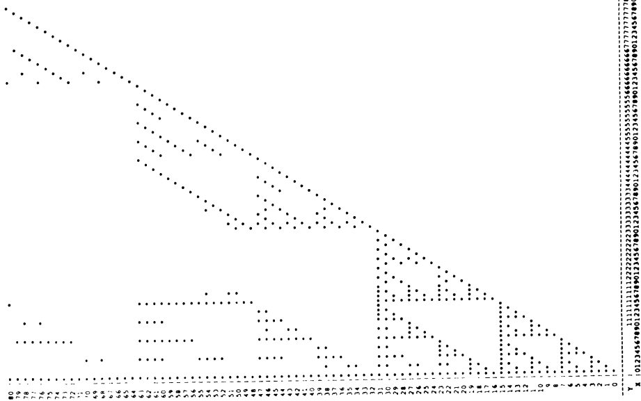
19-ary divisors
