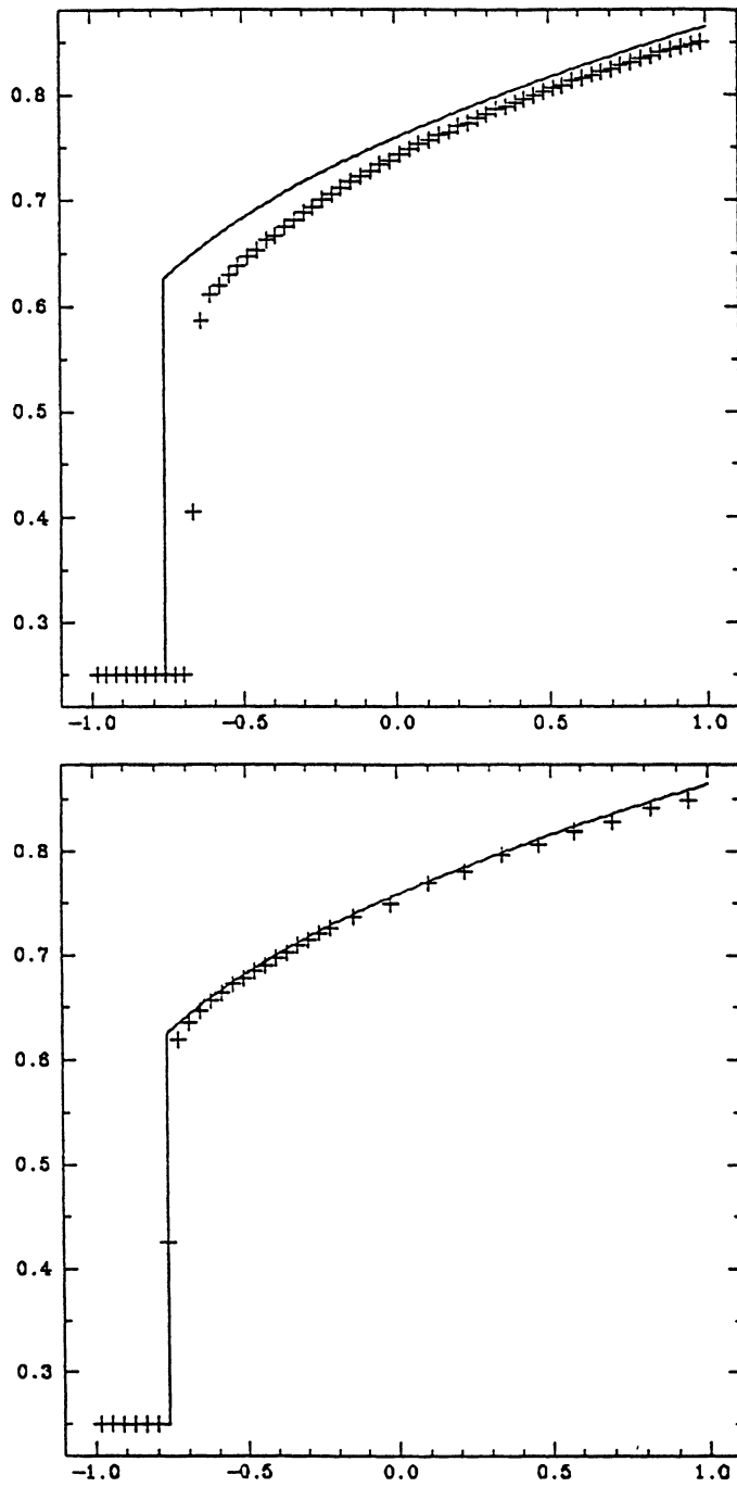
FIGURE 10. Initial-boundary value problem (3.3). Cut along the diagonal.
