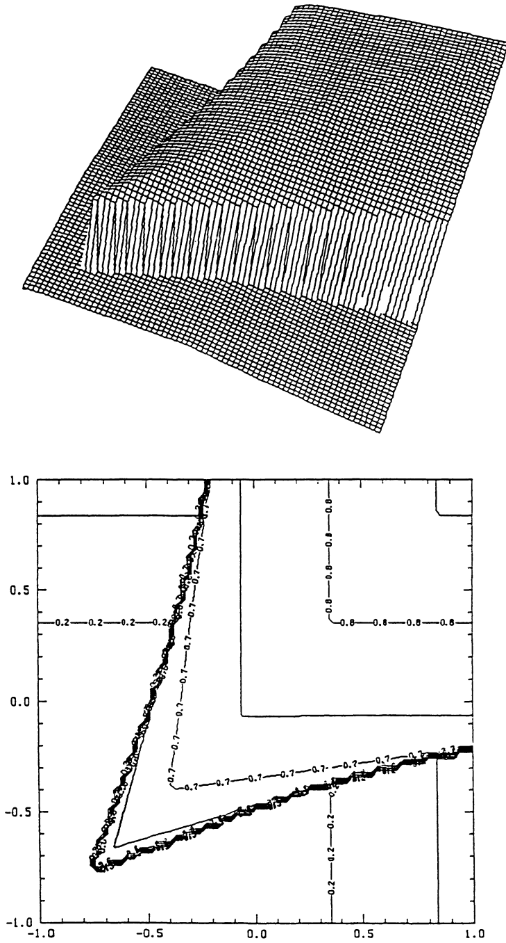
FIGURE 7. The exact solution. Initial value problem (3.3), T = 1 .
