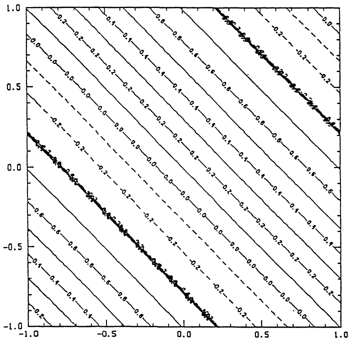
FIGURE 4. The exact solution. Initial value problem (3.1), T = 0.45 .
