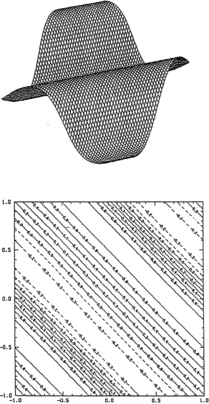
FIGURE 2. The exact solution. Initial value problem (3.1), T = 0.1 .
