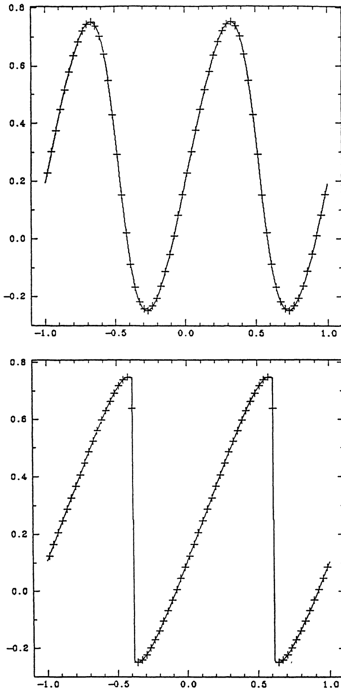
FIGURE 6. Initial value problem (3.1). Cut along the diagonal. Top: T = 0.1 , bottom: T = 0.45 .
