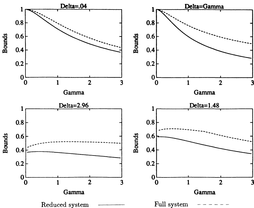
FIGURE 4.9. Asymptotic bounds for the block Jacobi iteration matrices on four cross-sections of the (\gamma, \delta) plane, for upwind differences.
