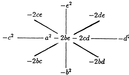
FIGURE 4.2. The computational molecule for the reduced system.
