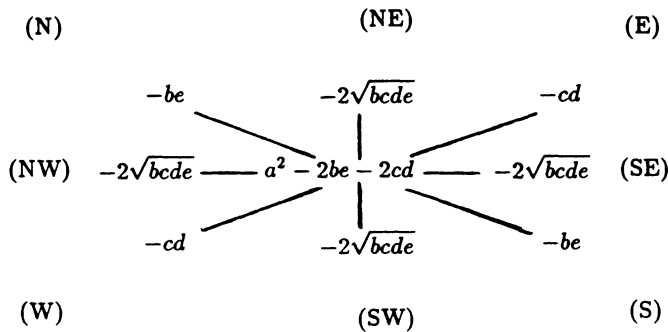
FIGURE 4.5. A computational molecule for the rectilinear periodic reduced operator.
