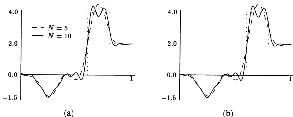
FIGURE 3 Comparison of algorithm and Fourier series reconstruction by algorithm using Fourier cosine series
