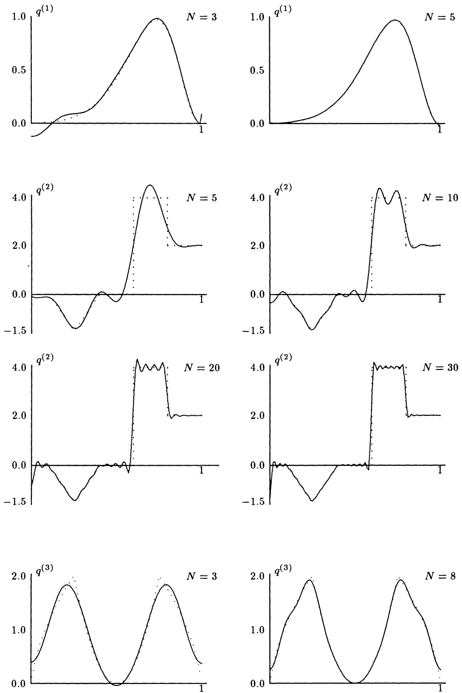
FIGURE 2 Reconstruction of q(x) for various values of N
