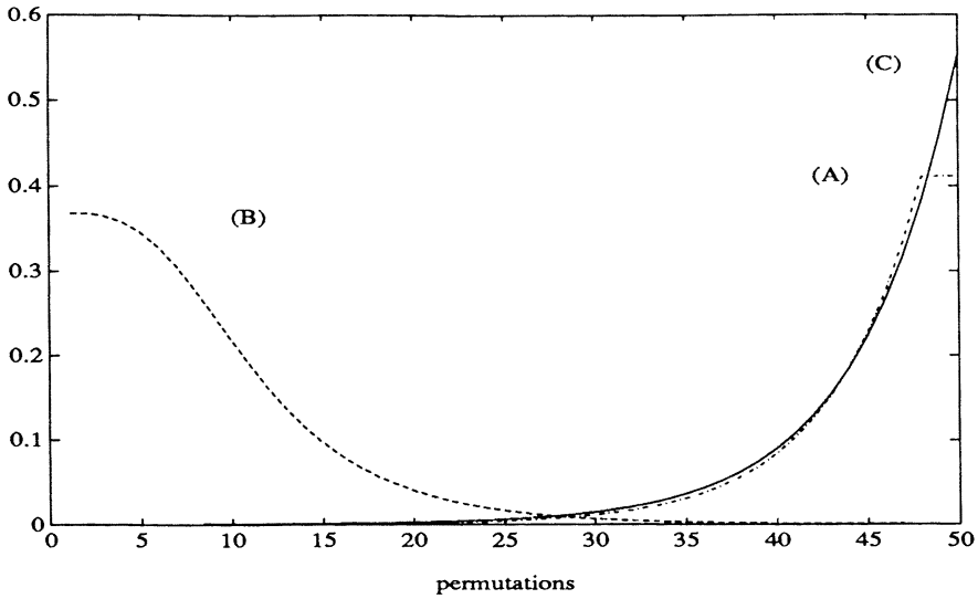
FIGURE 1. Kahan's example
