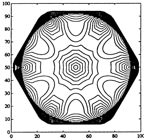
FIGURE (6.5) Contour lines, for values 1, 1.05, ..., 2, of Lebesgue function for interpolation at hexagon points and their center
