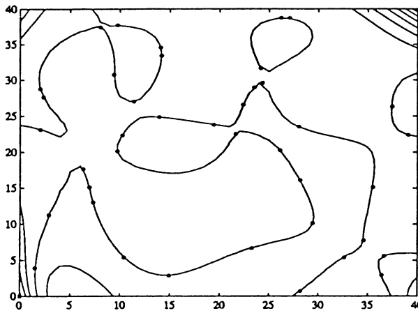
FIGURE (6.6) Contour lines for error in interpolation at 40 random points
