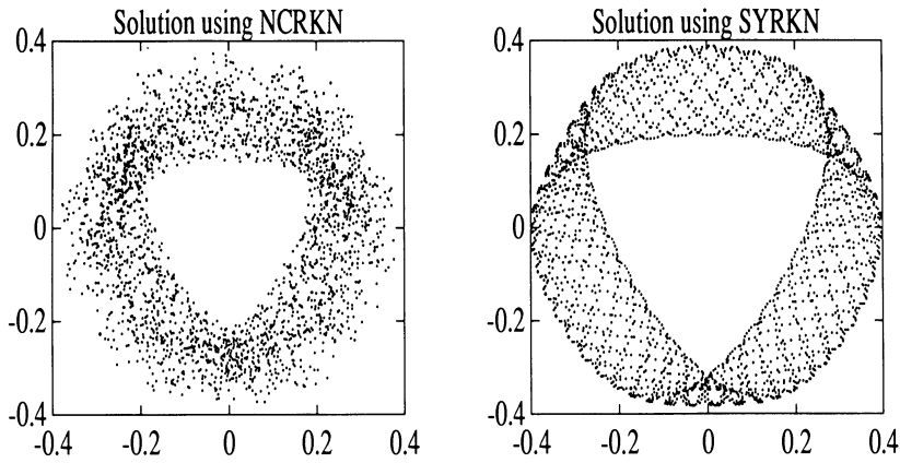
FIGURE 3. Trajectories for the Hénon-Heiles problem using canonical and noncanonical methods ( H = 0.117835 )
