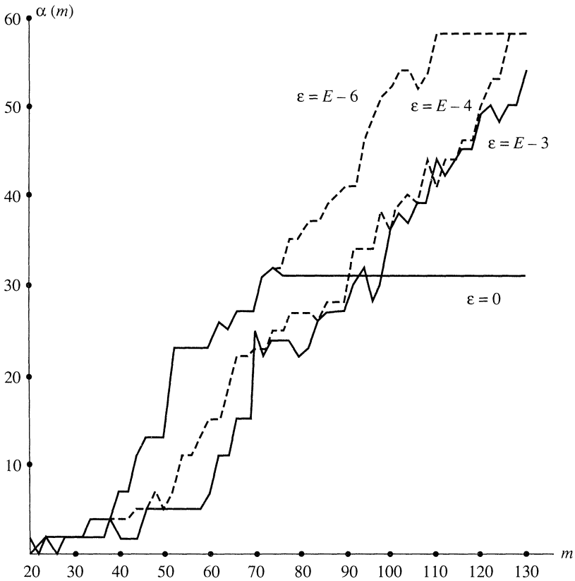
FIGURE 2. Convergence results of 130 steps for the 500 \times 500 random matrix of Example 8.4 with rebiorthogonalization
