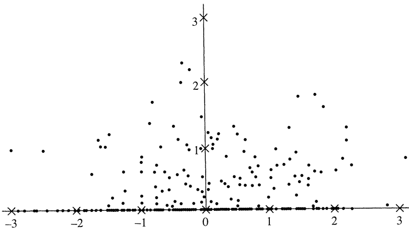
FIGURE 4. The distribution of the eigenvalues in Example 8.4
