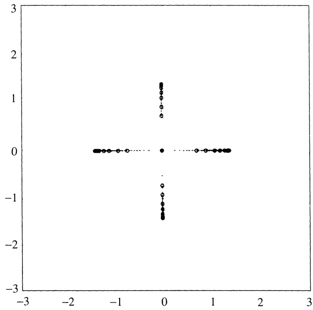
FIGURE 3. Zeros of F_n(z) for 4-star when n = 31
