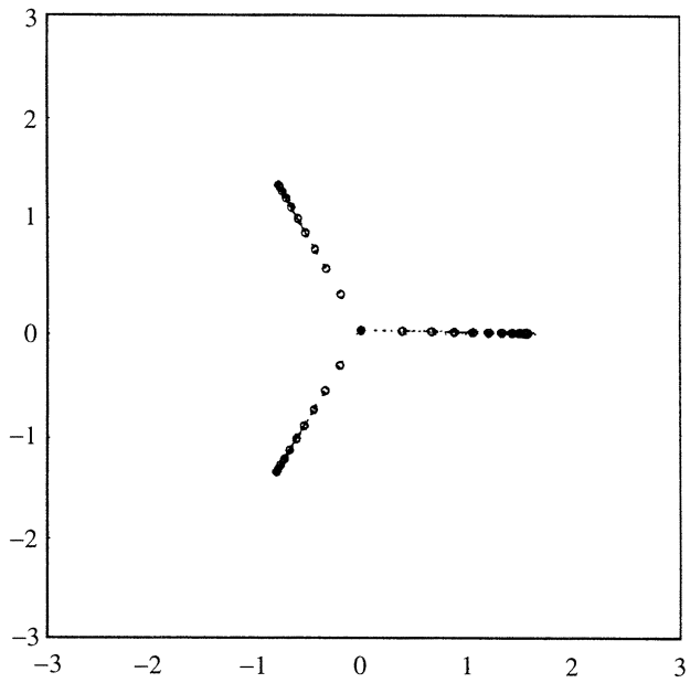
FIGURE 1. Zeros of F_n(z) for 3-star when n = 31
