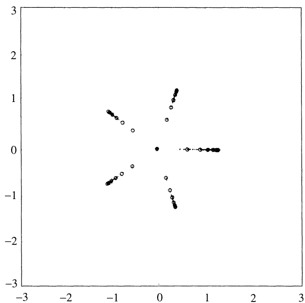
FIGURE 5. Zeros of F_n(z) for 5-star when n = 31
