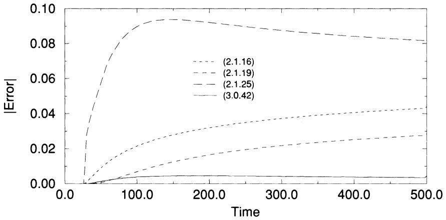
FIGURE 4. Errors for n = 0 , \omega = 1 , R = 16
