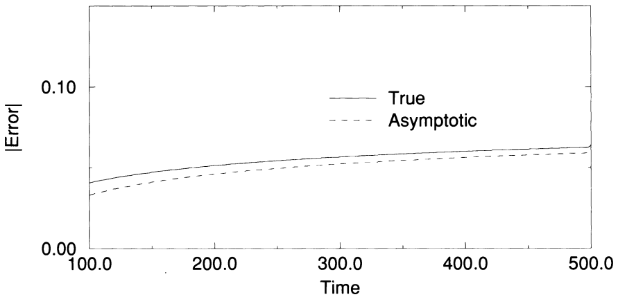
FIGURE 5. Asymptotic expansion vs. true error, condition (2.1.25)
