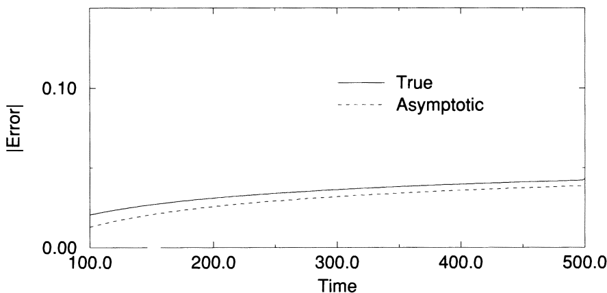
FIGURE 6. Asymptotic expansion vs. true error, condition (2.1.16)
