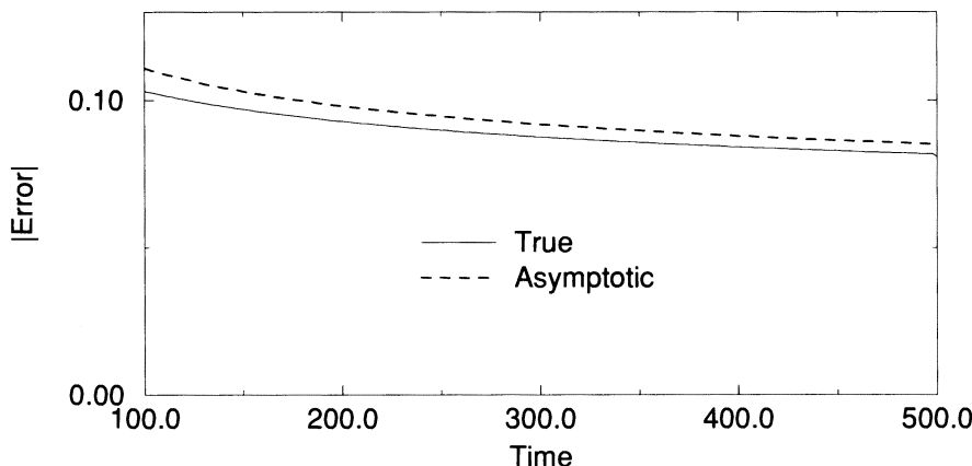
FIGURE 7. Asymptotic expansion vs. true error, condition (2.1.19)
