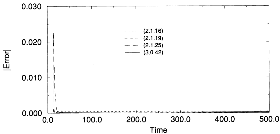
FIGURE 9. Errors for n = 2 , \omega = 1 , R = 8
