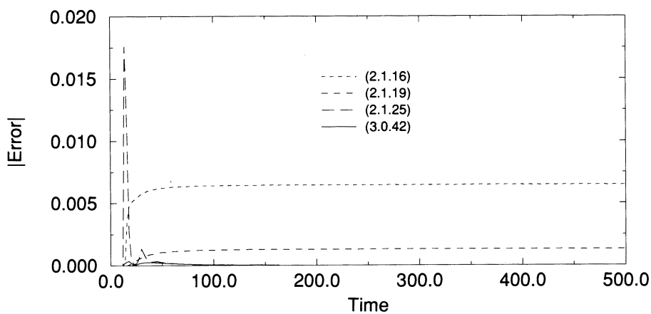
FIGURE 8. Errors for n = 1 , \omega = 1 , R = 8
