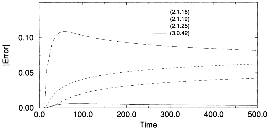
FIGURE 1. Errors for n = 0 , \omega = 1 , R = 8
