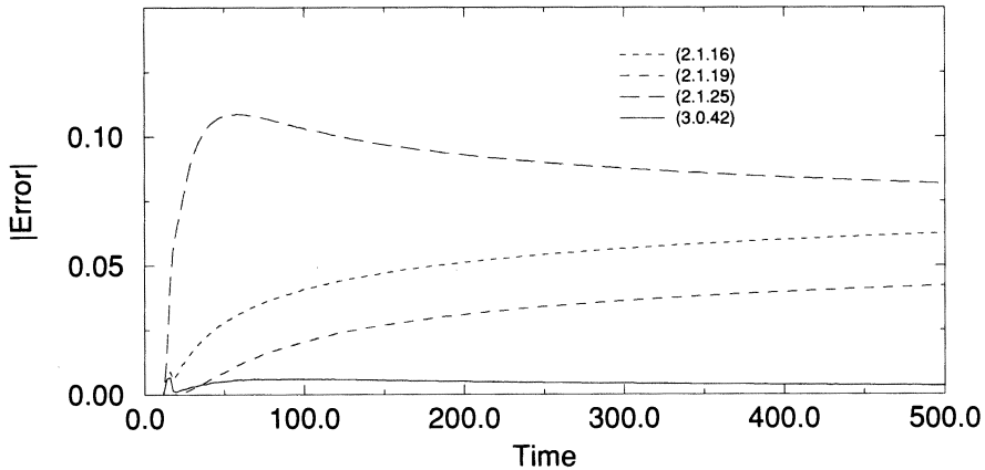
FIGURE 2. Errors for n = 0 , \omega = 4 , R = 8
