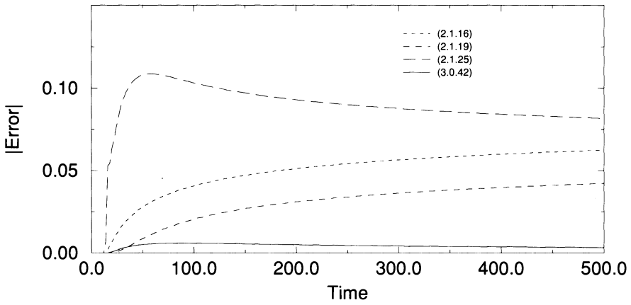
FIGURE 3. Errors for n = 0 , \omega = \frac{1}{2} , R = 8
