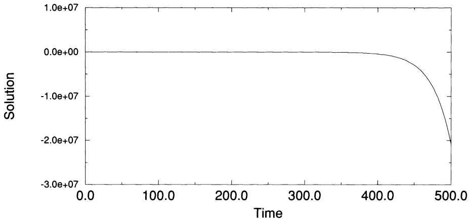
FIGURE 11. Solution at r = 1.8 using (2.1.28), n = 0 , \omega = 1 , R = 8
