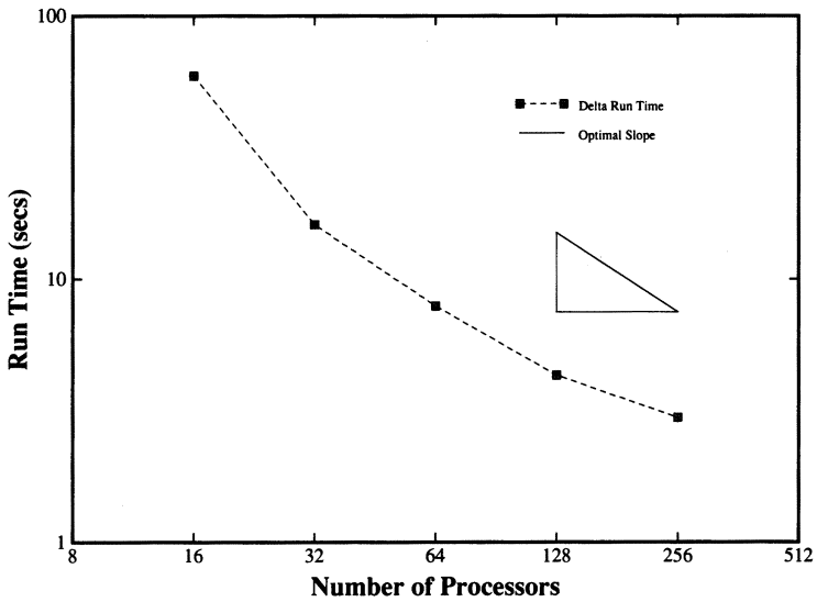
FIGURE 6. Scaling of the BDD algorithm
