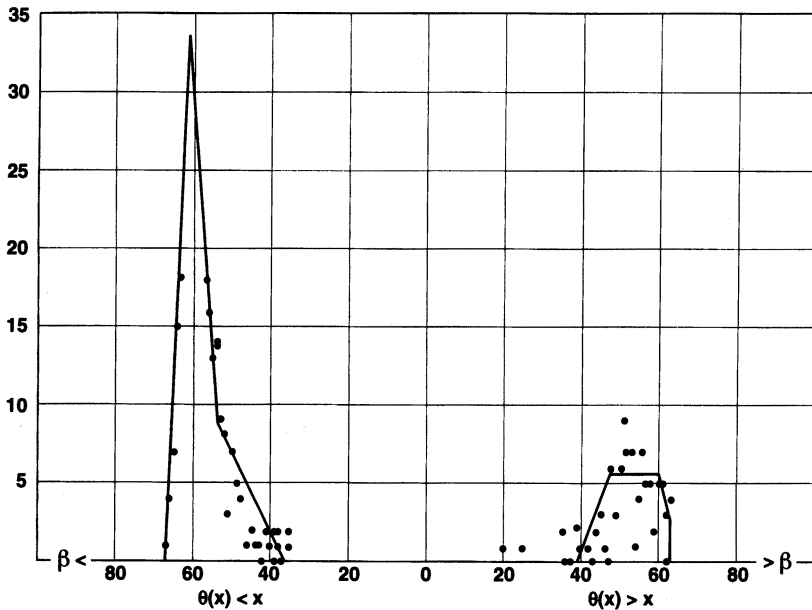
FIGURE 7. Histogram. Remainder = |\theta(x) - x| = x^\beta ; 800 \leq trace number \leq 1200
