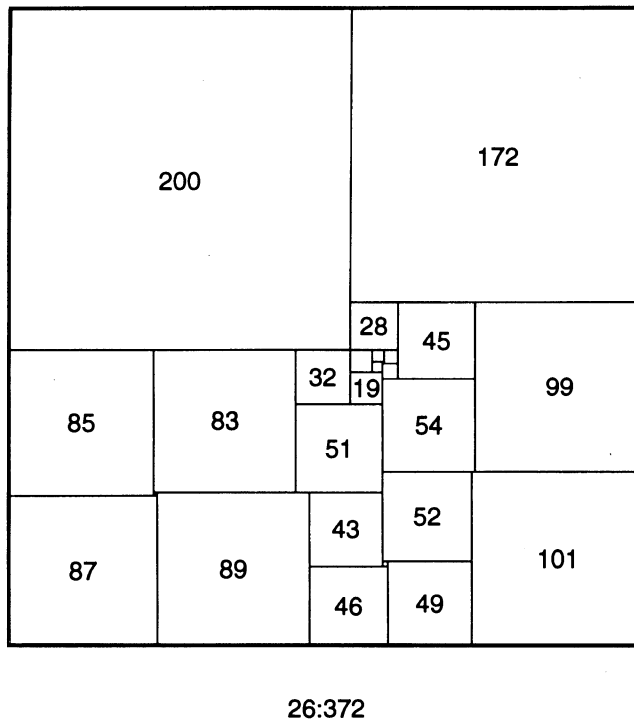
FIGURE 3. Simple perfect squared square of order 26 with a cross
