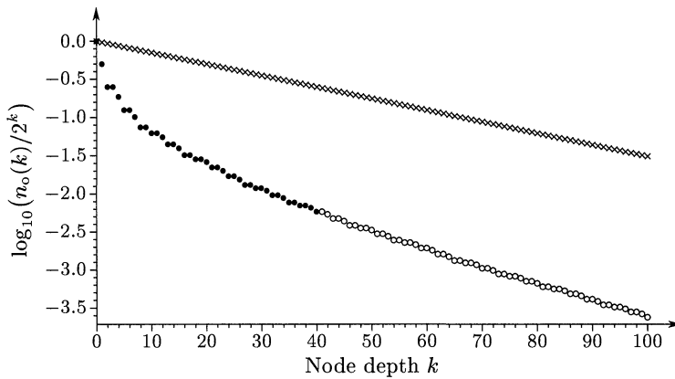
FIGURE 3. This linear-log graph depicts the ratio between open nodes at depth k of the search tree, and the total number of nodes ( 2^k ) at that same depth. Shaded circles (●) represent exact values (generated by our program), open circles (○) represent values computed with the recurrence formulas described in the appendix, and crosses (×) represent the upper bound of 1 - F(k) given by Theorem D of [3].
