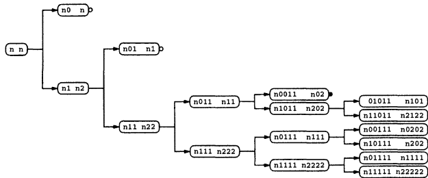
FIGURE 2. The search tree for 0 \leq k \leq 5 . A small open circle ( \circ ) after a node indicates a cycle (for n_k = 0 ). A small shaded circle ( \bullet ) after a node indicates that the stopping time for the congruence class of initial values associated with that node is exactly equal to that node's depth. These two types of nodes do not need to be subdivided. Only the nodes with maximal depth (and without a circle) are used in the search.
