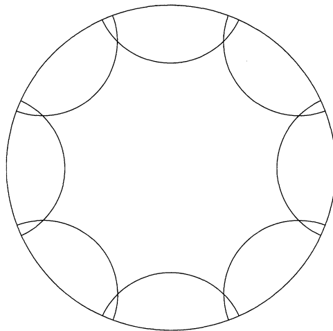
FIGURE 2. The regular octagon.
