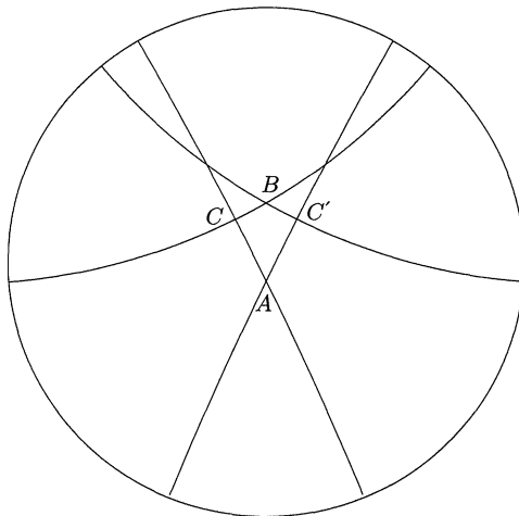
FIGURE 3. Fundamental domain in the case of a maximal order in (\omega, -1)_{\mathbb{Q}(\omega)} , where \omega is the positive root of x^3 + 2x^2 - x - 1 = 0 .
