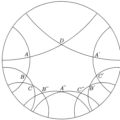
FIGURE 1. Fundamental domain in the case of a maximal order in (1 + \sqrt{2}, -3)_{\mathbb{Q}(\sqrt{2})} .
