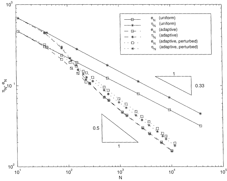
FIGURE 5. Error and error estimator for uniform, adaptive, and perturbed adaptive mesh-refinement in the nonconforming finite element scheme in Example 7.1.
