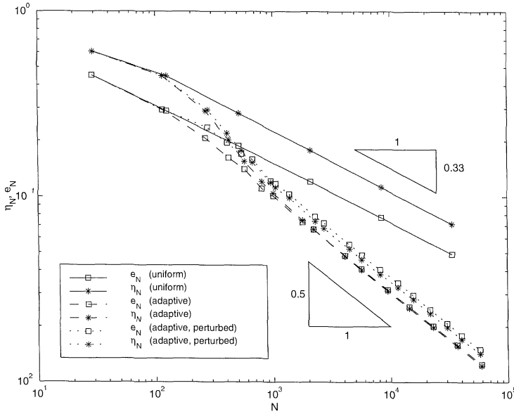
FIGURE 7. Error and error estimator for uniform, adaptive, and perturbed adaptive mesh-refinement in the mixed finite element scheme in Example 7.1.
