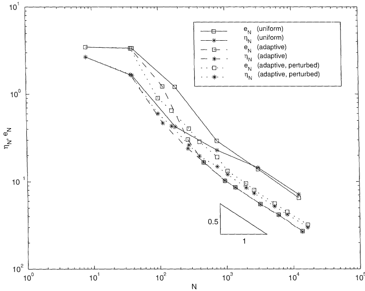
FIGURE 6. Error and error estimator for uniform, adaptive, and perturbed adaptive mesh-refinement in the nonconforming finite element scheme in Example 7.2.
