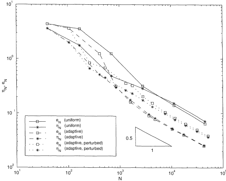
FIGURE 8. Error and error estimator for uniform, adaptive, and perturbed adaptive mesh-refinement in the mixed finite element scheme in Example 7.2.
