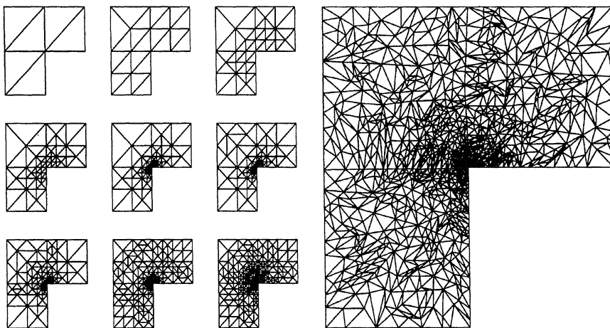
FIGURE 1. Adaptively refined meshes \mathcal{T}_0 (left upper) to \mathcal{T}_8 (right lower) (left) and perturbed triangulation \mathcal{T}_{16} with 1157 free nodes (right) in Example 7.1 for the conforming finite element scheme.
