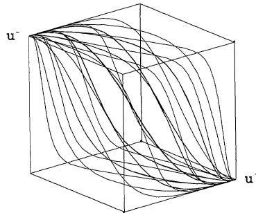
FIGURE 1. Some orbits from the three-dimensional manifold connecting u^- and u^+ .
