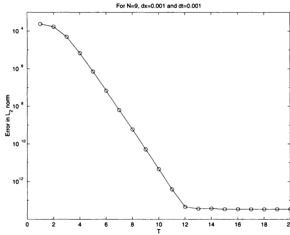
FIGURE 2. The l^2 -error in time for Example 5.2.
