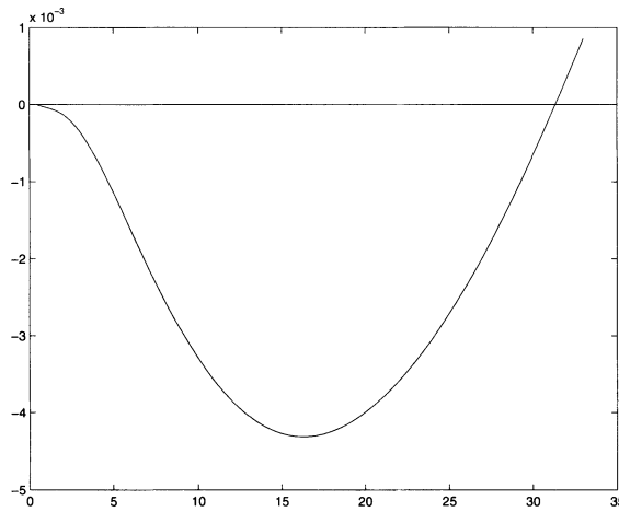
FIGURE 1. Graph of F_\gamma(\log(\frac{z}{z_0})) for r_1 = 1 , r_2 = 2 and \gamma = 1.27
